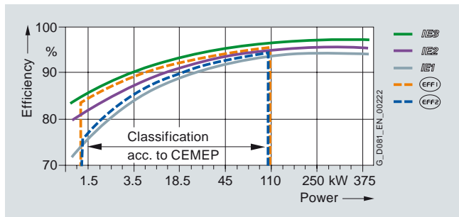
IE1 to IE3 efficiencies 4-pole 50 Hz
