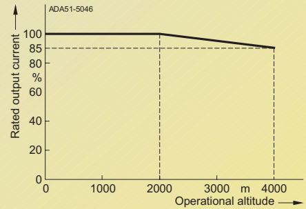
Inverter 90 kW to 200 kW
