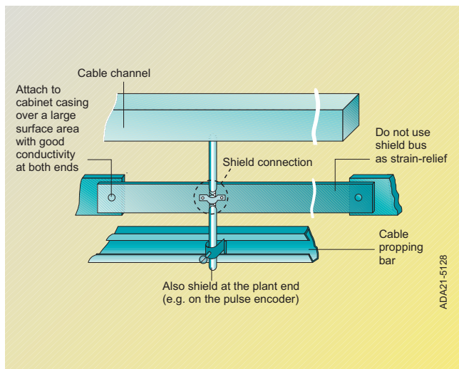
Fig. 5/37 Shielding with routing into the cabinet
