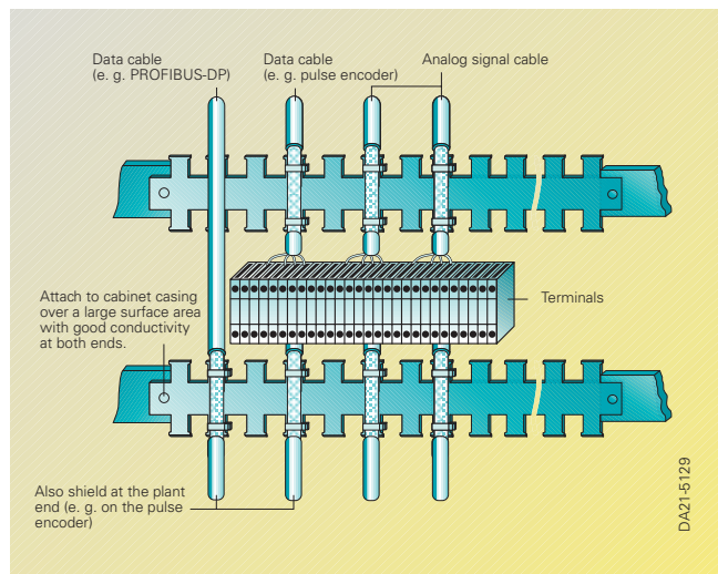
Fig. 5/38 Shielding in the cabinet
