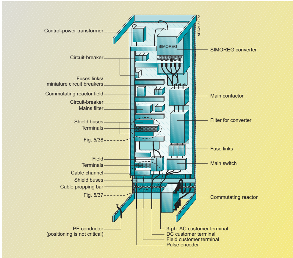
Fig. 5/36 Example of cabinet arrangement with a SIMOREG converter
