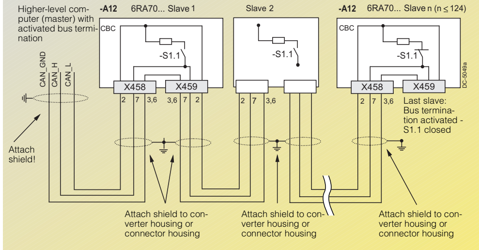
Fig. 4/26 Data exchange between CBC boards with bus interruption
