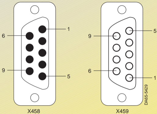
Fig. 4/29 X458 (plug) and X459 (socket) connections
