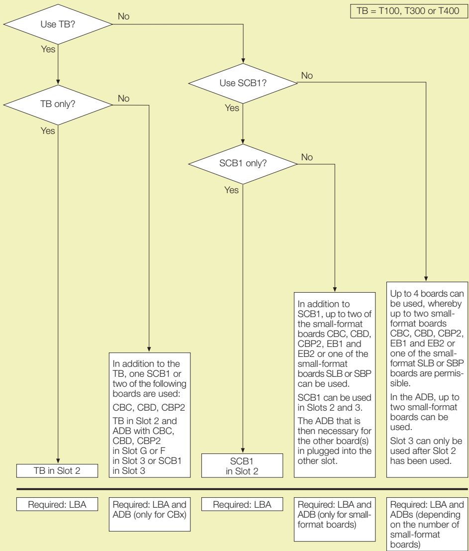
Possible locations or slots for supplementary boards as well as their possible combinations
