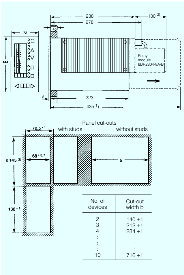
Fig. 1 SIPART DR24 multi-function unit and panel cut-outs, dimensions
