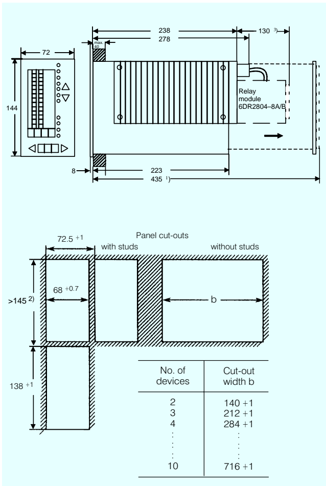
Fig. 1 SIPART DR22 controller and panel cut-outs, dimensions
